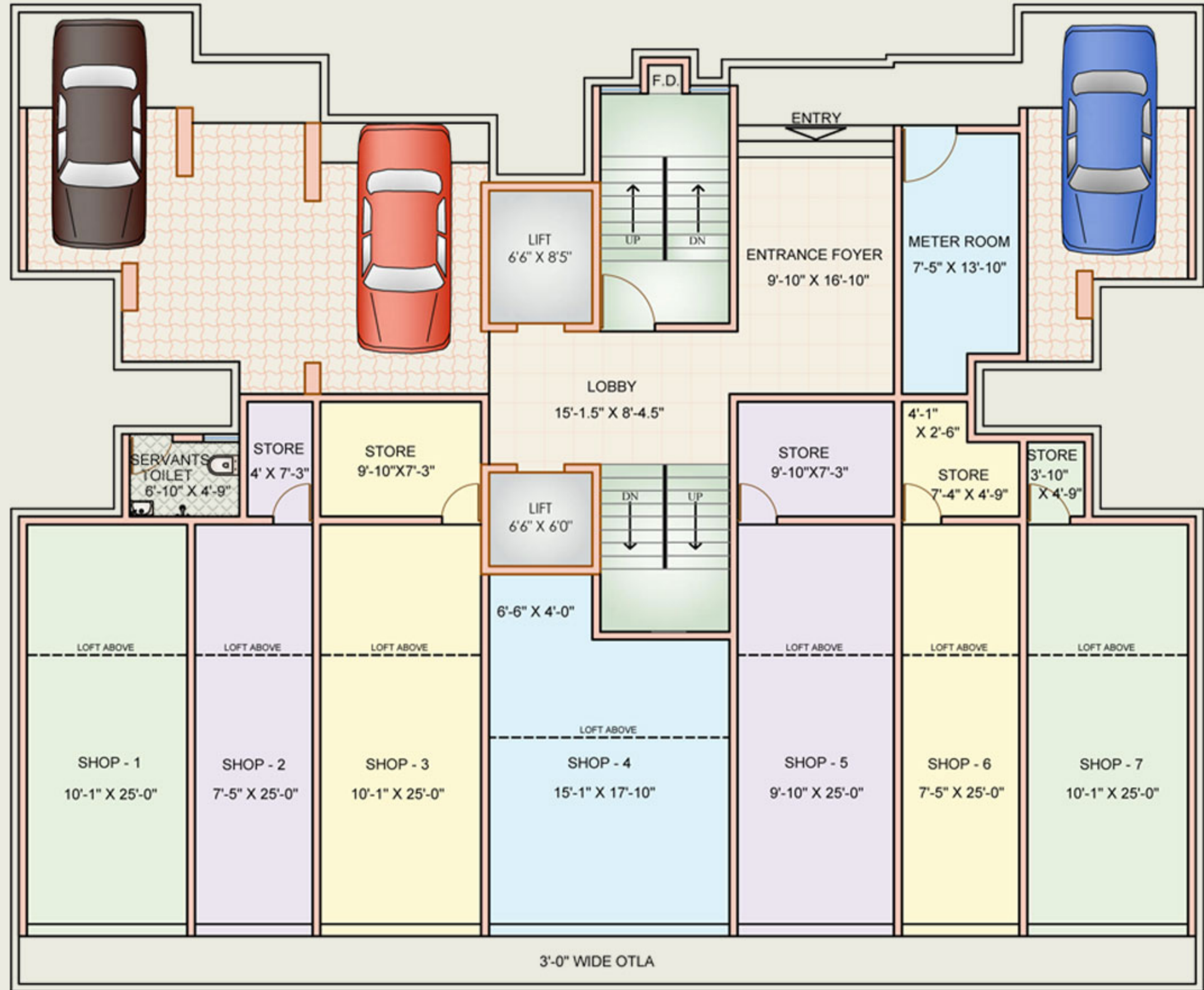
CHARMS HEIGHTS (FINEZE) - GROUND FLOOR, A-2
